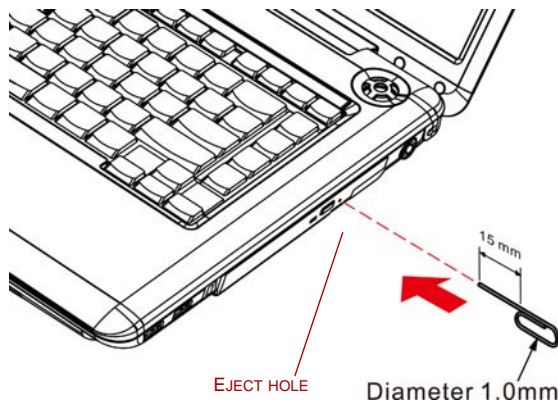
Figure 4-4 Manual release with the eject hole
